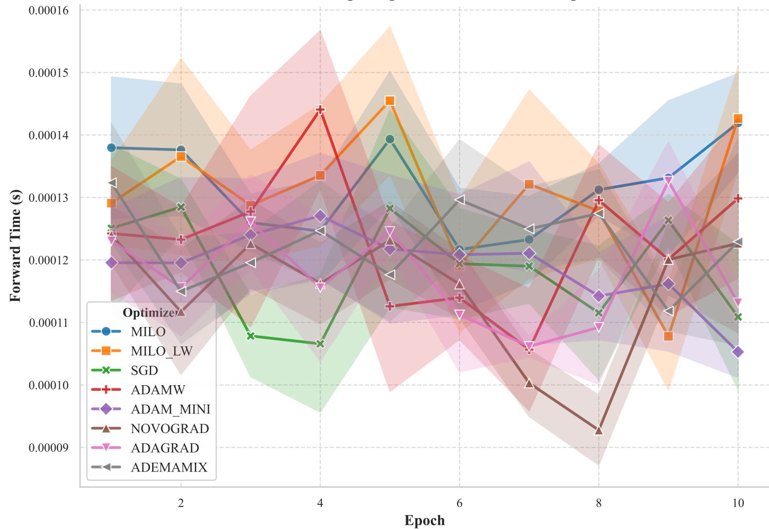
Forward Runtime per Epoch for LOGISTIC Experiment
